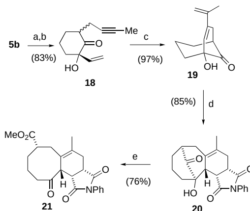
Scheme 8. Synthesis of the stereochemically-rich 8-6 bicarbocycle 21 : a) \text{CH}_2\text{CHLi} , THF, -78^\circ\text{C} , then 1-bromo-2-butyne; b) TBAF (1.2 equiv), THF, 30 min, 20^\circ\text{C} ; c) 3 (5 mol %), \text{CH}_2\text{Cl}_2 , 40^\circ\text{C} , 3 h; d) N -phenylmaleimide, toluene, sealed tube, 155^\circ\text{C} , 5 h; e) \text{Pb}(\text{OAc})_4 , MeOH, 20^\circ\text{C} , 5 min.
