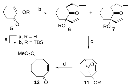
Scheme 4. Synthesis of cyclooctenone 12 : a) TBSCl, imidazole, \text{CH}_2\text{Cl}_2 ; b) \text{CH}_2\text{CHLi} , THF, -78^\circ\text{C} , then allyl bromide; c) 3 (5 mol %), \text{CH}_2\text{Cl}_2 , 40^\circ\text{C} ; d) \text{Pb}(\text{OAc})_4 , MeOH, 20^\circ\text{C} .
