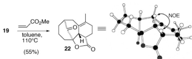
Scheme 9. Diels–Alder reaction of 19 with methyl acrylate.
