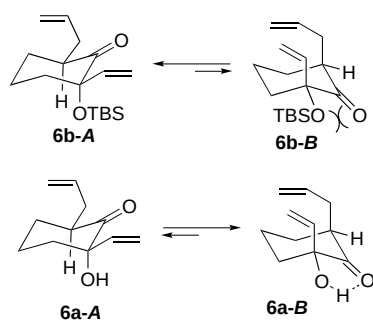
Figure 1. Proposed conformational equilibria, corroborated by simple MM2 calculations. [8]
