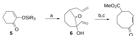
Scheme 2. Strategy for constructing the required cyclooctanoid ring: a) 1) \text{CH}_2\text{CHLi} , THF, -78^\circ\text{C} , then allyl bromide; 2) TBAF, THF; b) 3, \text{CH}_2\text{Cl}_2 , 20^\circ\text{C} ; c) \text{Pb}(\text{OAc})_4 , MeOH, 20^\circ\text{C} .
