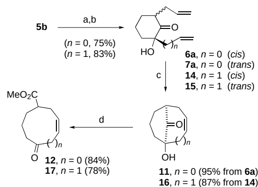
Scheme 7. Best protocol for the synthesis of cyclooctenone 12 and cyclononone 17 : a) \text{CH}_2\text{CHLi} (for 12 ) or \text{CH}_2\text{CHCH}_2\text{Li} (for 17 ), THF, -78^\circ\text{C} , then allyl bromide; b) TBAF (1.2 equiv), THF, 30 min 20^\circ\text{C} ; c) 3 (5 mol %), \text{CH}_2\text{Cl}_2 , 20^\circ\text{C} ; d) \text{Pb}(\text{OAc})_4 (1.5 equiv), MeOH, 20^\circ\text{C} , 5 min.
