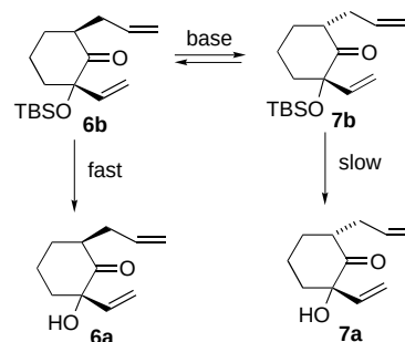
Scheme 6. Hypothesized isomerization–kinetic desilylation process.
