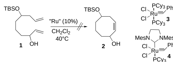
Scheme 1. Unsuccessful attempts at RCM of 1 .
