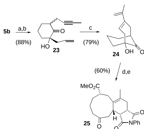
Scheme 10. Synthetic approach to the stereochemically rich fused 9–6 bicarbocycle 25 : a) \text{CH}_2\text{CHCH}_2\text{Li} , THF, -78^\circ\text{C} , then 1-bromo-2-butyne; b) TBAF (1.2 equiv), THF, 20^\circ\text{C} , 30 min; c) 3 (5 mol%), \text{CH}_2\text{Cl}_2 , 40^\circ\text{C} , 5 h; d) N -phenylmaleimide, toluene, sealed-tube, 160^\circ\text{C} , 4 h; e) \text{Pb}(\text{OAc})_4 , MeOH, 20^\circ\text{C} , 5 min.
