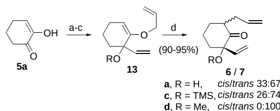
Scheme 5. Synthesis of cyclohexanones 6 and 7 by Claisen rearrangement: a) Allyl alcohol, p -TsOH, benzene; b) \text{CH}_2\text{CHMgBr} , THF, -78^\circ\text{C} , then \text{H}_3\text{O}^+ ; c) for 13c : TMS-imidazole, \text{CH}_2\text{Cl}_2 , for 13d : NaH, THF, 0^\circ\text{C} , then MeI; d) toluene, sealed tube, 160^\circ\text{C} .
