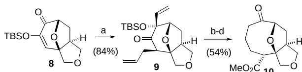
Scheme 3. Strategy for ring enlargement of the oxabicyclic pyrone-alkene cycloadducts: a) \text{CH}_2\text{CHLi} , THF, -78^\circ\text{C} , then allyl bromide; b) 3 (5 mol %), \text{CH}_2\text{Cl}_2 , 40^\circ\text{C} ; c) \text{H}_2 , Pd/C; d) 1) TBAF, THF; 2) \text{Pb}(\text{OAc})_4 , MeOH, sealed tube, 100^\circ\text{C} , 1 h.
