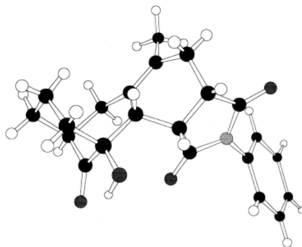
Figure 2. Representation of the structure of compound 20 , as determined by X-ray crystallography.
